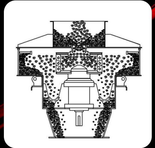
CV Type with Rockshelf CV Malzeme Yastıklı Tip
