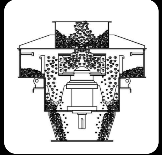
CV Type with Anvils CV Çarpma Takozlu Tip
